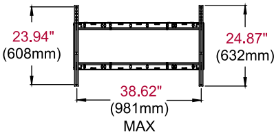
ADAPTOR BRACKET
